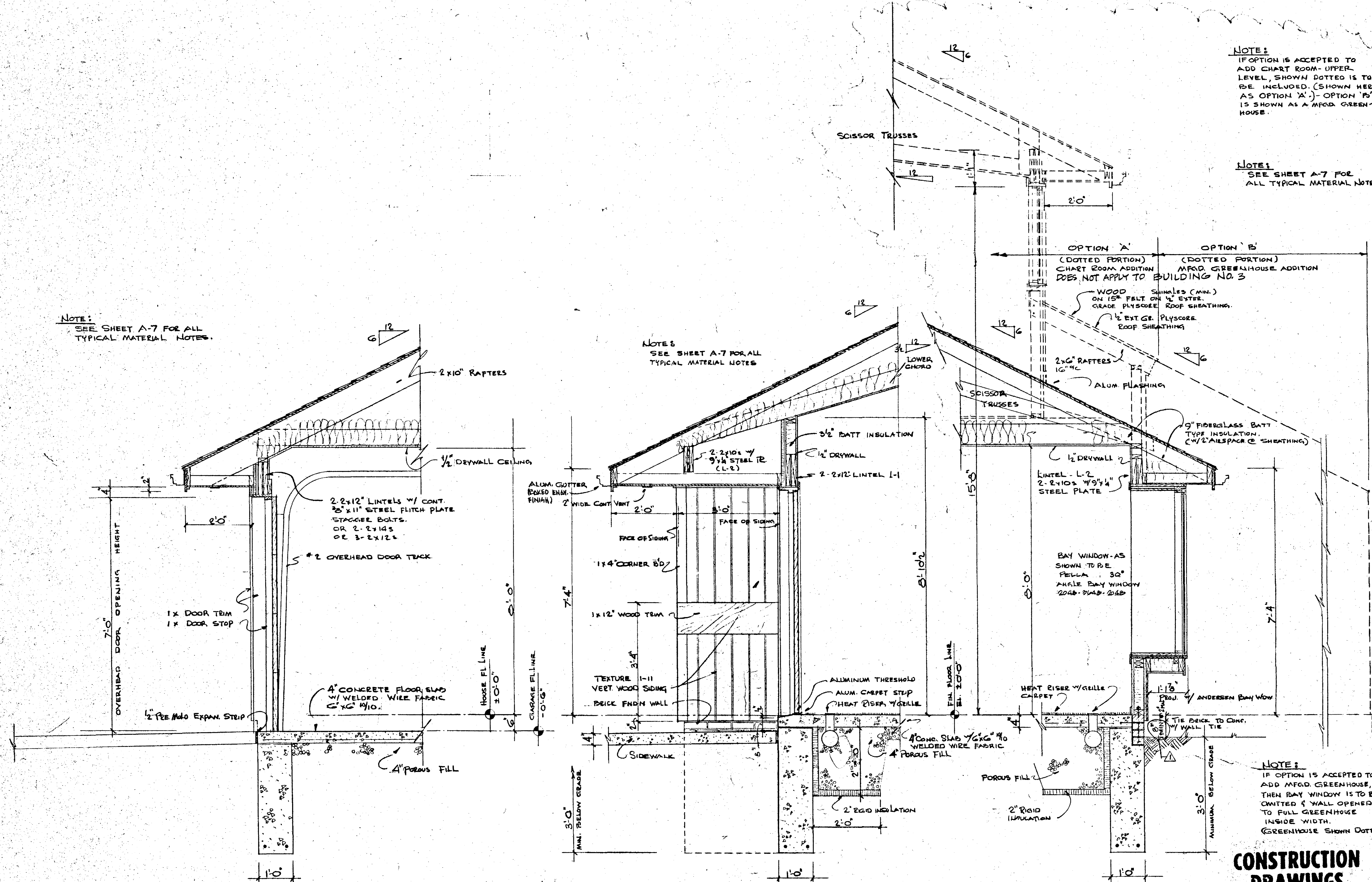
SECTION C SCALE 3/4"=1'-0"
